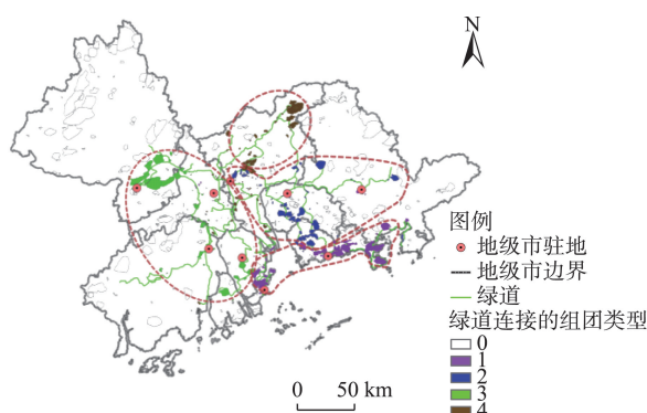
图3 珠三角城市群区域绿道连接的拓扑网络 Fig.3 Topological network connected by greenways in the Pearl River Delta region
